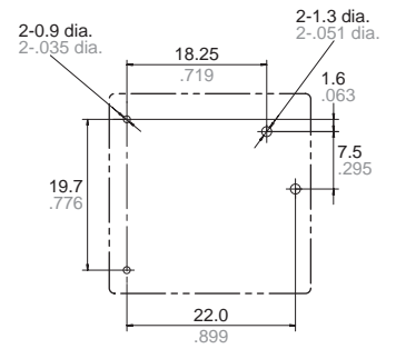
PC board pattern (Bottom view)
