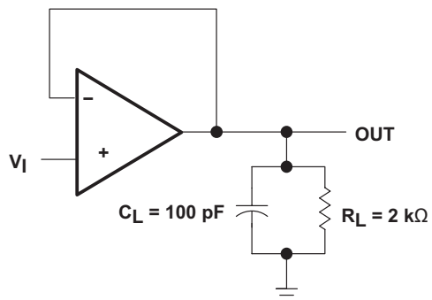
Figure 4. Unity-Gain Amplifier
