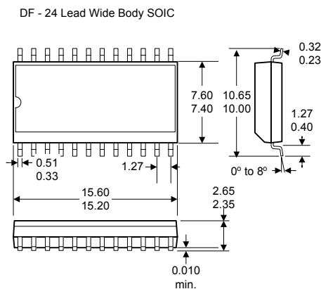
Figure 5: Package information
