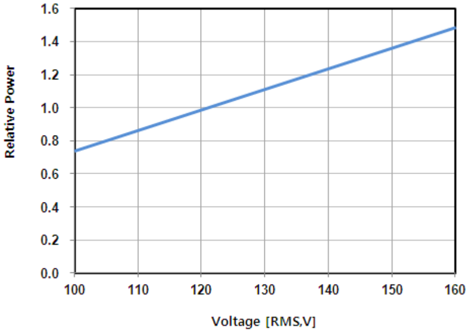
Fig 4. Relative Power Distribution vs. Voltage, T_a = 25^\circ\text{C} , 120V
