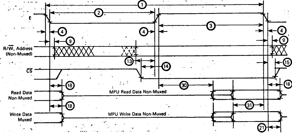
FIGURE 3 - BUS TIMING
