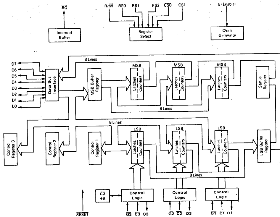
FIGURE 2 - BLOCK DIAGRAM
