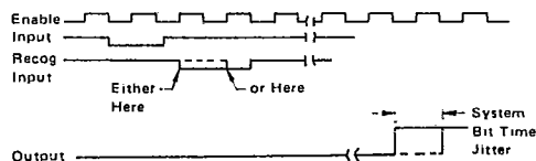
FIGURE 11 — INPUT JITTER
