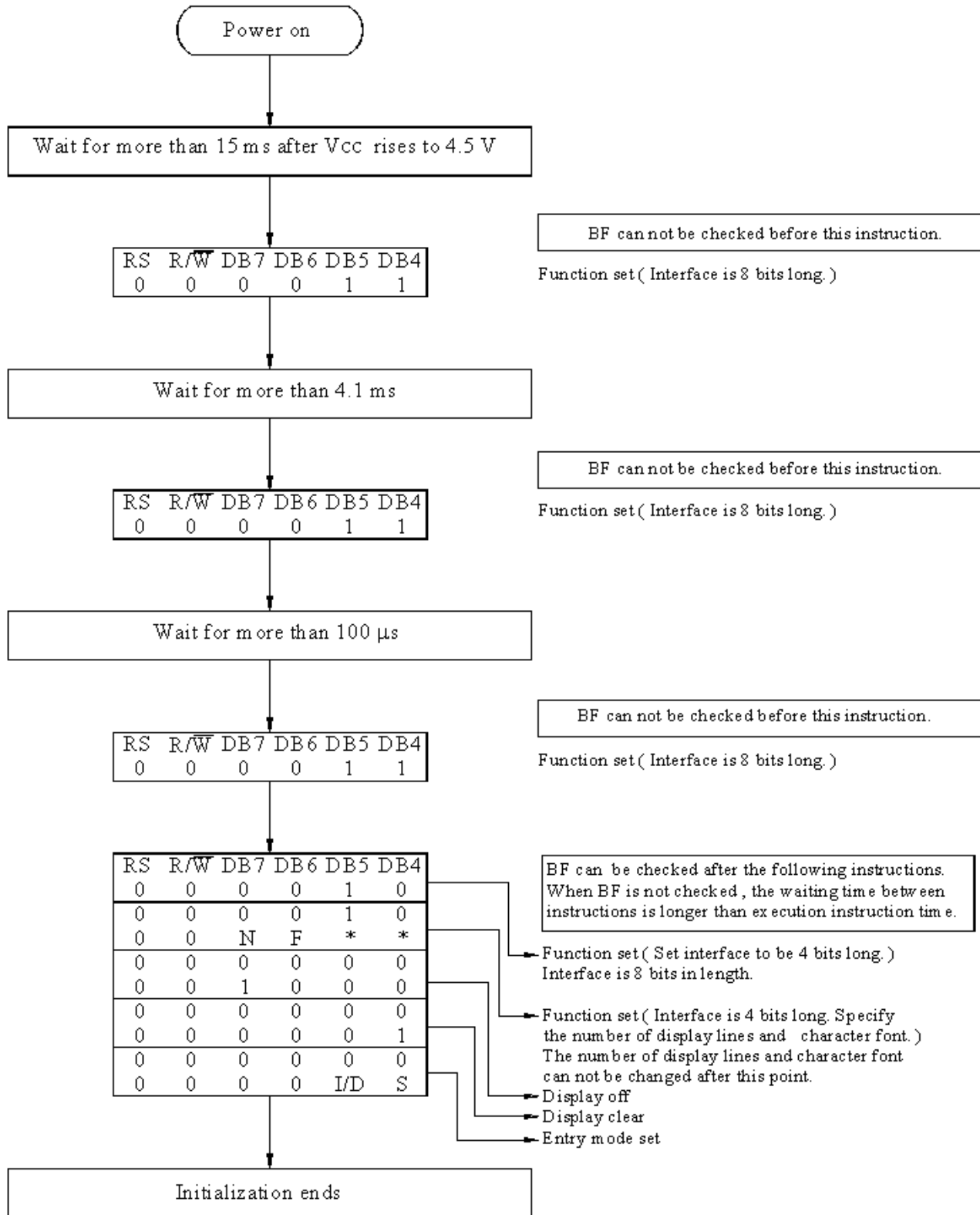
4-Bit Interface
