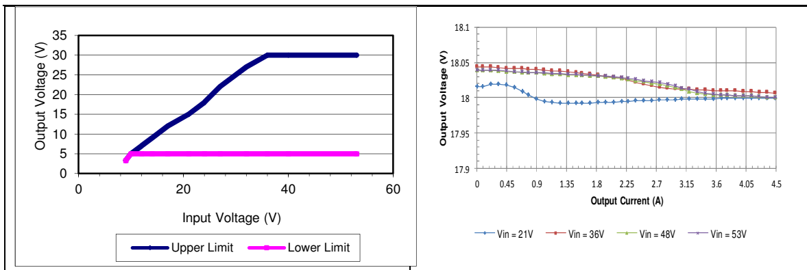
Output Voltage versus Input Voltage Operating Range
