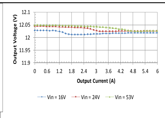
V_o=12V Typical load regulation
