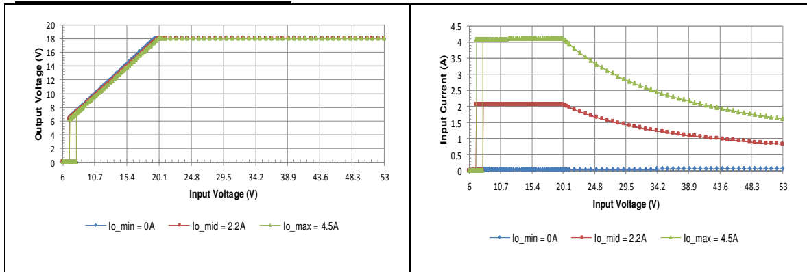
Vo=18V Typical Output Voltage vs. Input Voltage Characteristics
