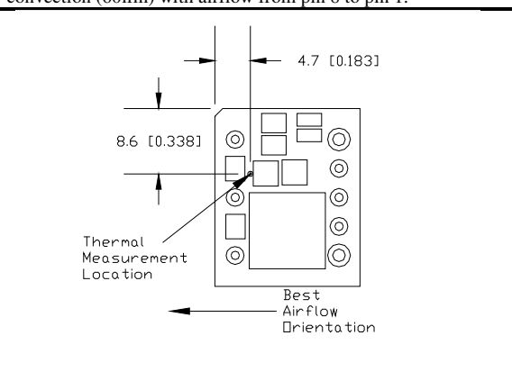
i3A4W005A150V thermal measurement location – top view
