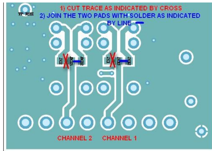
Rear PCB layer of the Receiver
