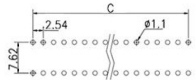
PCB Layout
