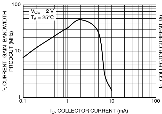
Figure 4. Current-Gain-Bandwidth Product
