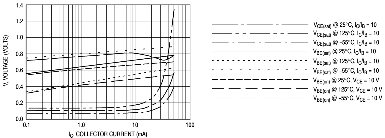
Figure 3. "ON" Voltages
