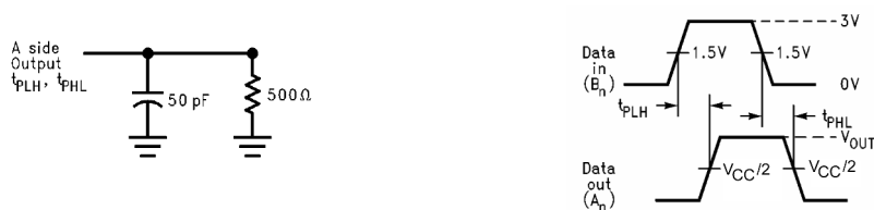
FIGURE 3. B to A Direction Test Load and Waveforms for Outputs A 1 - A 4
