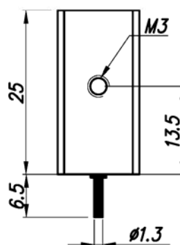
HR-95/25+PIN SOT32 36 K/W
