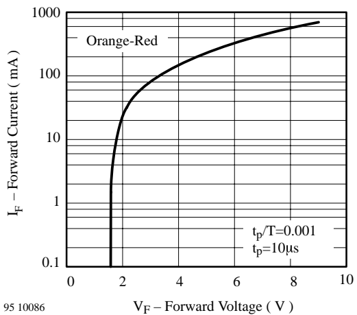
95 10086 Figure 9. Forward Current vs. Forward Voltage
