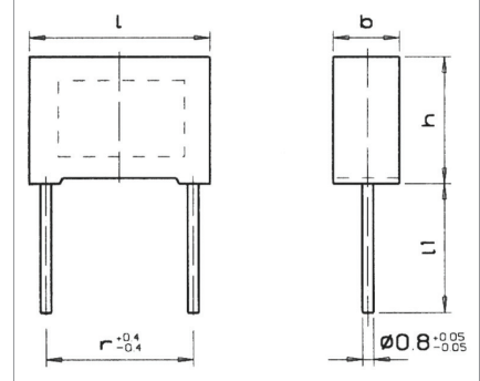
KLI1910 (dimensions in mm)
