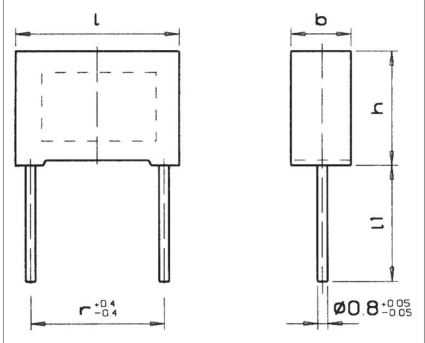
KNI1910 (dimensions in mm)
