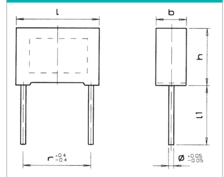
KNU1910 (dimensions in mm)
