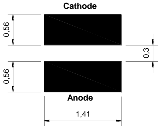
< Recommended Solder Pattern >
