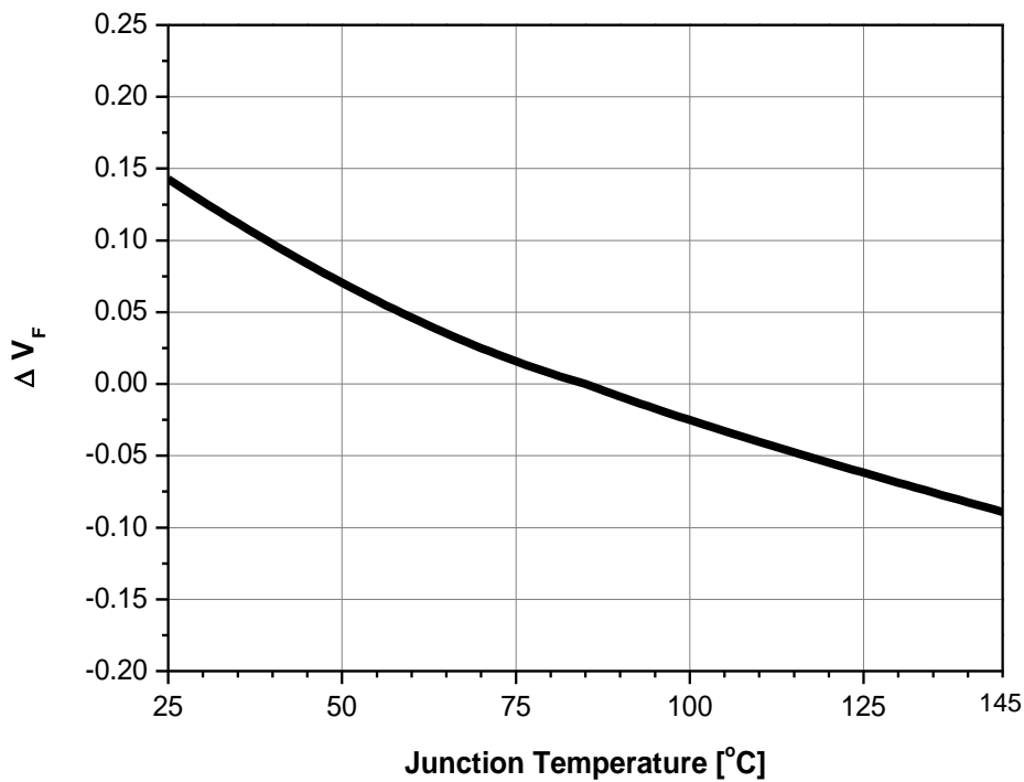
Fig 8. Relative Forward Voltage vs. Junction Temperature
